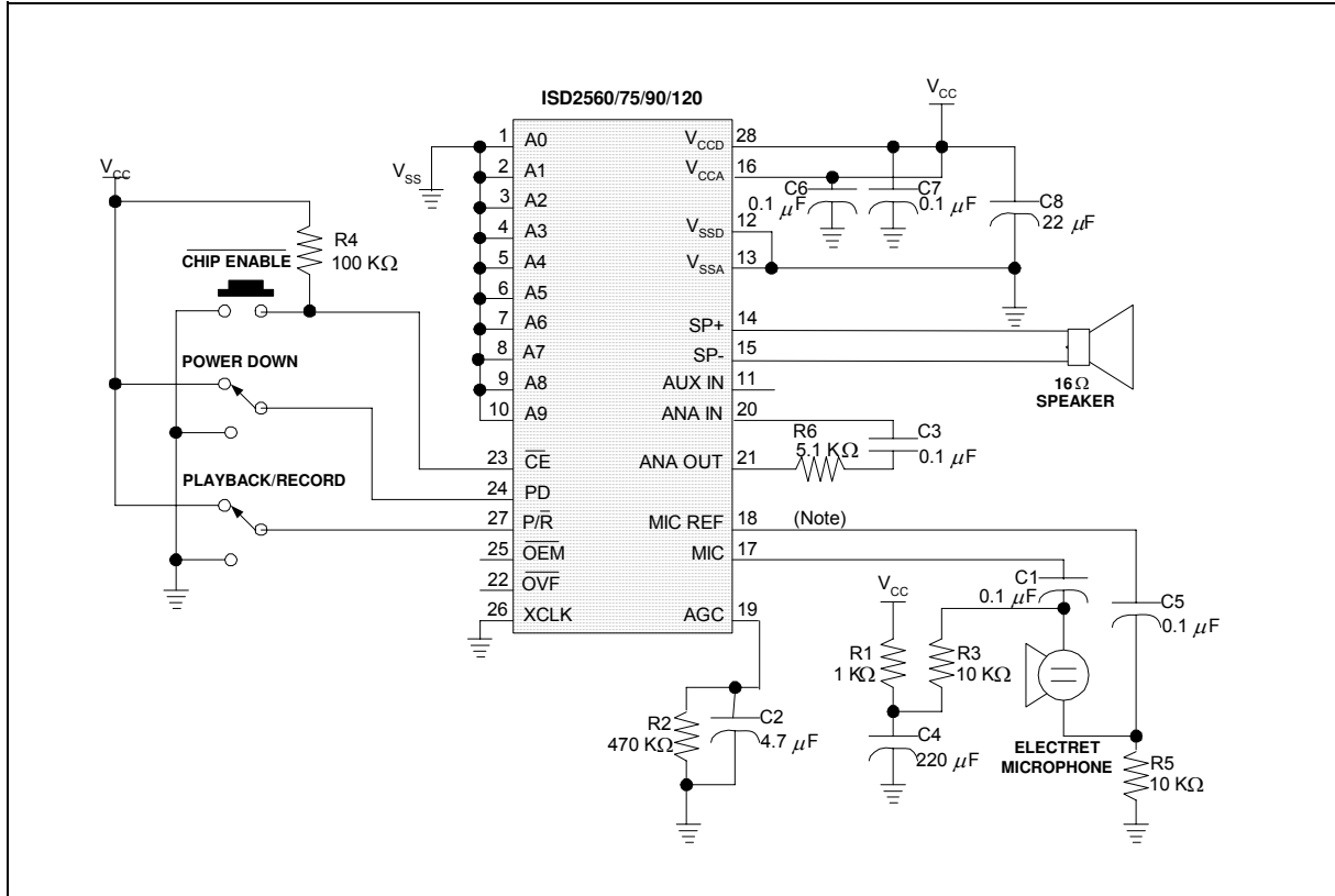
FIGURE 5: DESIGN SCHEMATIC
